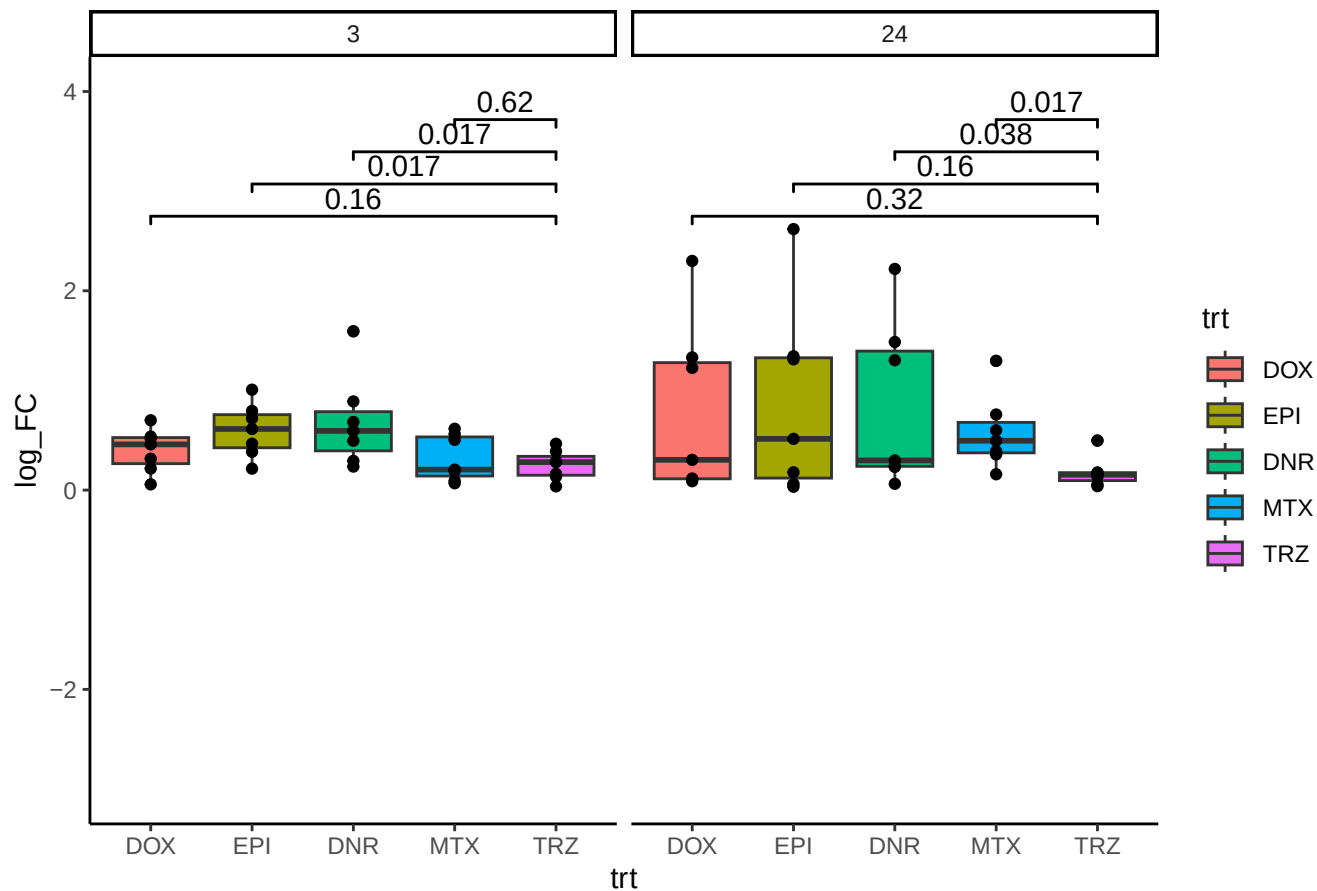
logFC of IHD overlapping regions, n = 7
